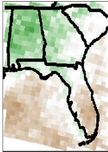
CGCM3/crcm
