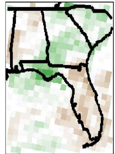
HadCM3/hrm3
