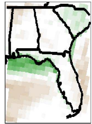
HadCM3/hrm3
