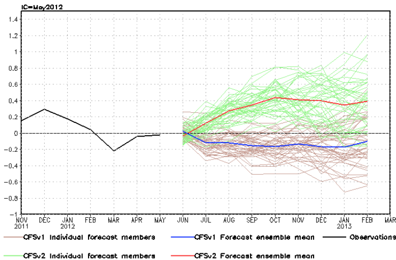
Tropical N. Atlantic SST anomalies (K)
