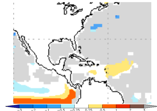
Skill masked SSTA for JJA2012
