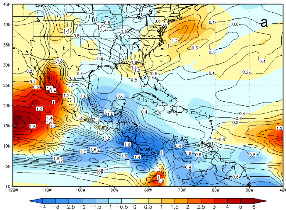
Precipitation (mm day -1 )
