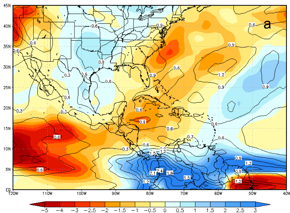
Precipitation (mmday -1 )
