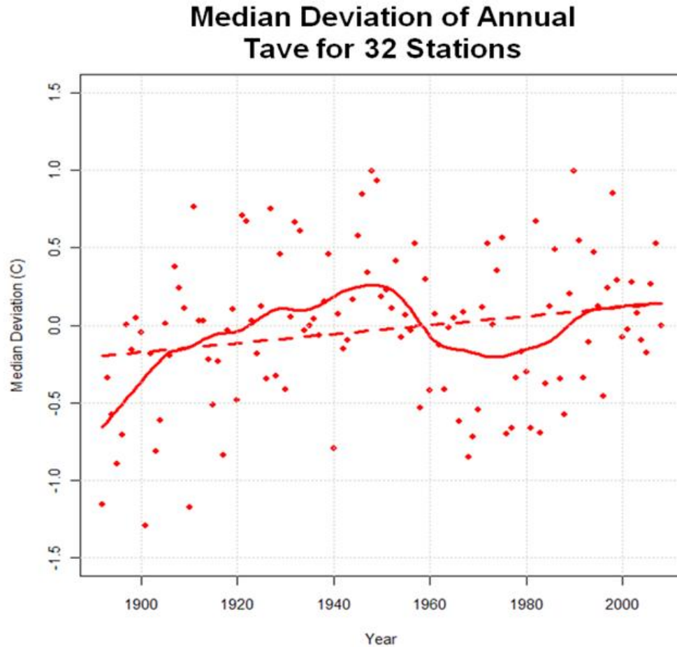
Figure 24. Median deviation of annual daily average temperature for the 32 stations in Florida. The dashed line represents the linear trend from OLS regression, while the solid line is the Lowess non-parametric regression line smoother which uses locally-weighted polynomial regression with a span of 0.25.
