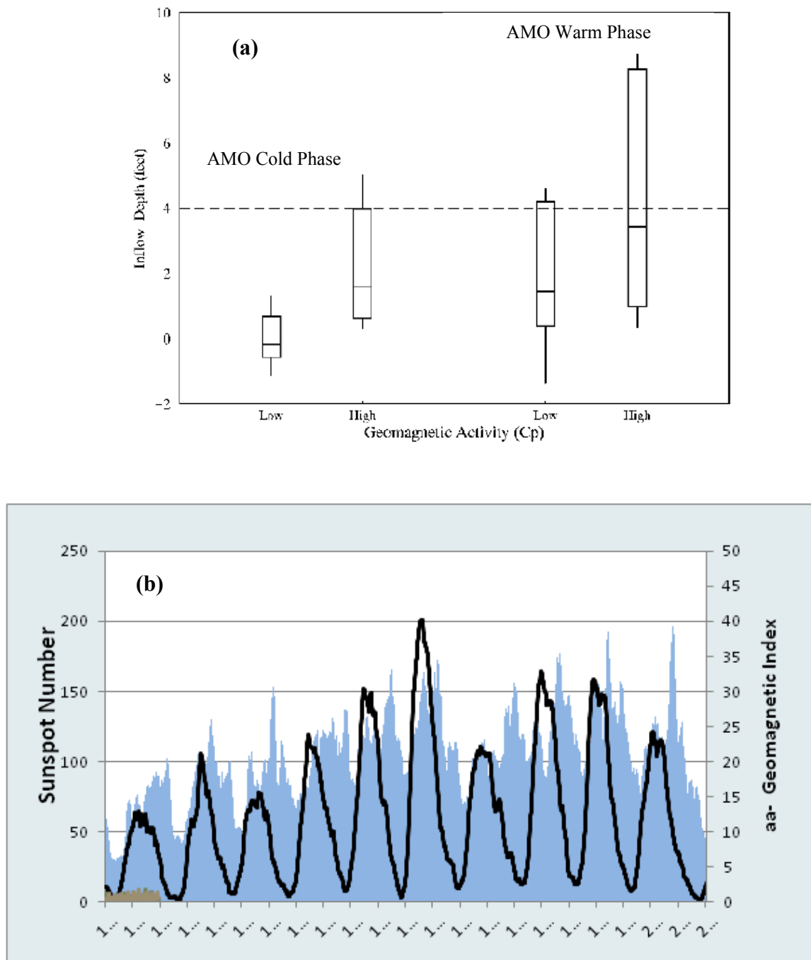
Figure 15/ (a) Lake Okeechobee net inflow versus solar activity (CP) and AMO. (b) Solar activity represented by sunspot number (black) and geomagnetic activity (blue) (Trimble, P. and Trimble, B. (1998).
