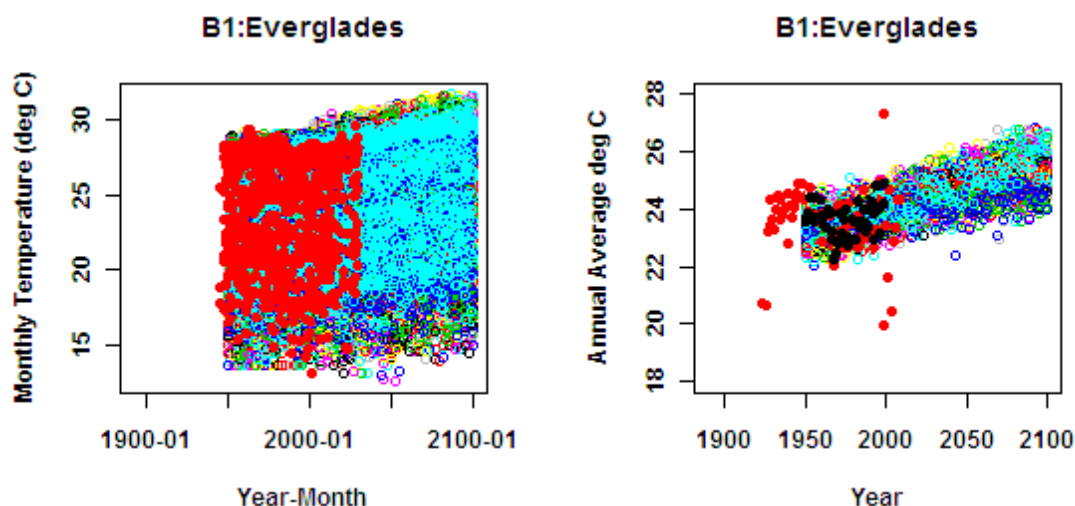
Figure 37. Monthly (left) and annual temperature patterns of BCSD models corresponding to the B1 scenario for the Everglades location. Also shown are historical observed (red dots) and historical simulated (black dots) for the same location.
