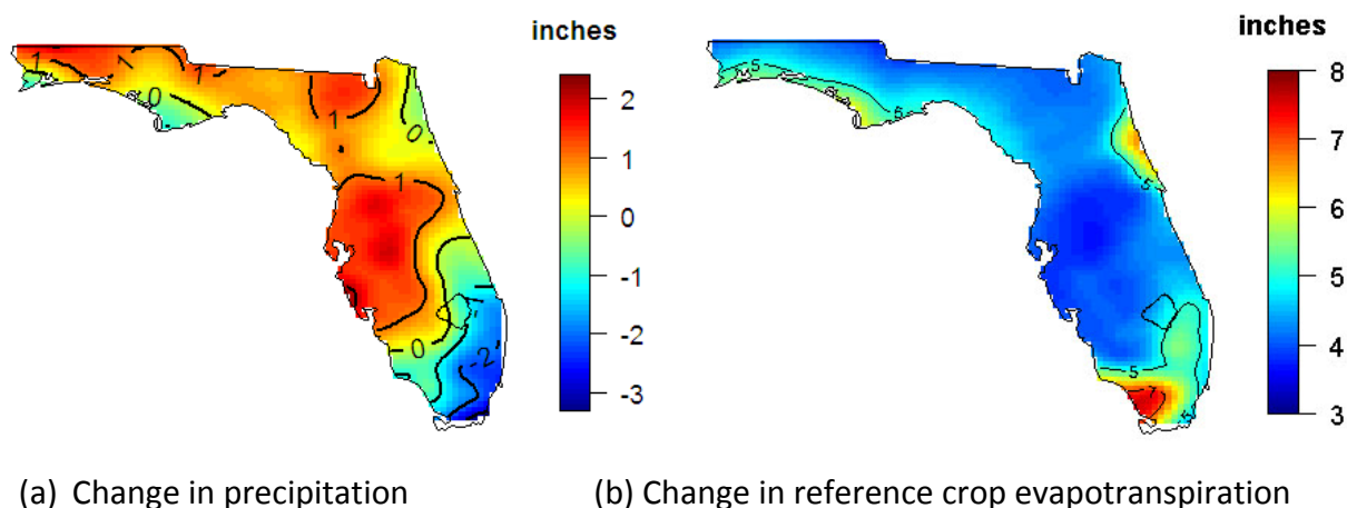
Figure 56. Change in precipitation and RET as predicted by CRCM circa 2050.
