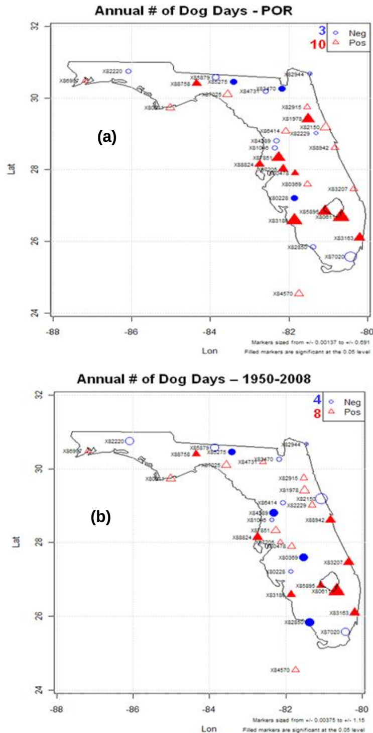
Figure 19. Trends in annual number of dog days for (a) the entire period of record, and (b) the 1950-2008 period. Triangles represent increasing trends, while circles represent decreasing trends. Filled markers represent trends significant at the 0.05 level.
