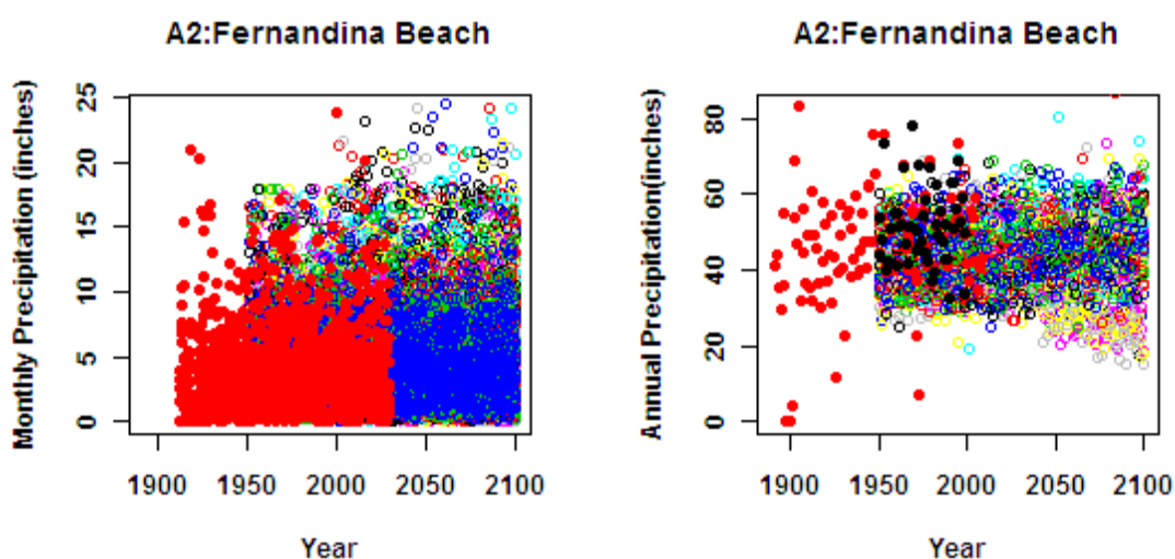
Figure 40. Monthly (left) and annual precipitation patterns of BCSD models corresponding to the A2 scenario for the Fernandina Beach location. Also shown are historical observed and simulated data for the same location (red and black dots, respectively).
