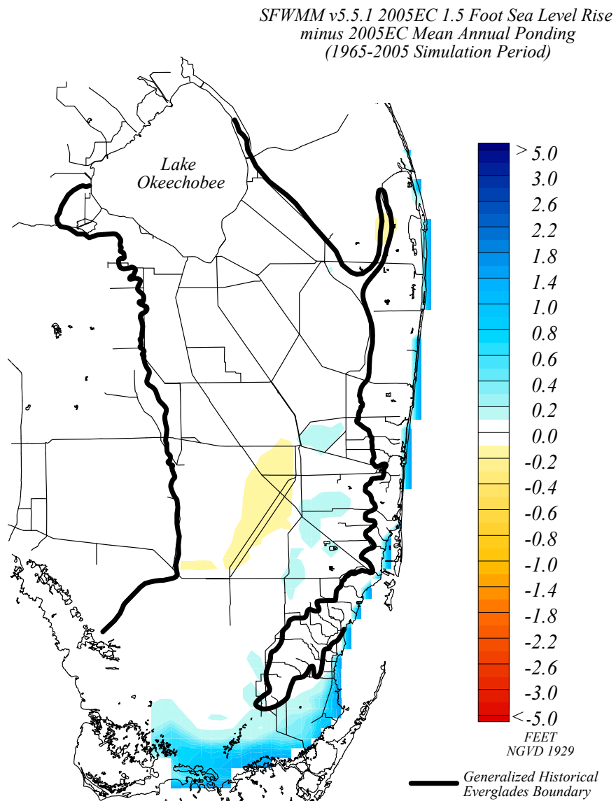
Figure 75. Average annual surface water ponding difference for the 2005 Existing Condition with 1.5 foot sea level rise minus the 2005 Existing Condition base run.
