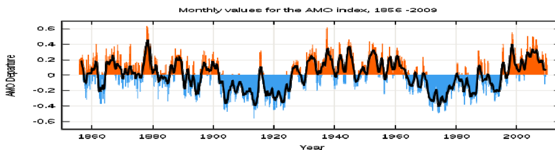
Figure 10. Atlantic Multi-decadal Oscillation. Departure from the Mean, Source: Enfield, D.B., A.M. Mestas-Núñez, and P.J. Trimble, 2001; Updated by Earth System Research Laboratory, Physical Science Division; Graphic Produced by Wikipedia: Atlantic Multi-decadal Oscillation.
