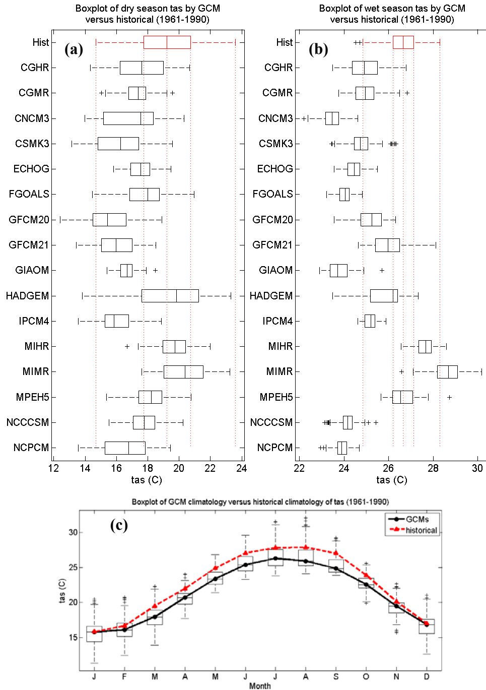
Figure 31. Comparison of the box-plots of GCM seasonal average temperature with that of the zonal dataset for(a) the dry season, and (b) the wet season; (c) comparison of the seasonal cycles of the observational temperature data with combined projections from all of the GCMs.
