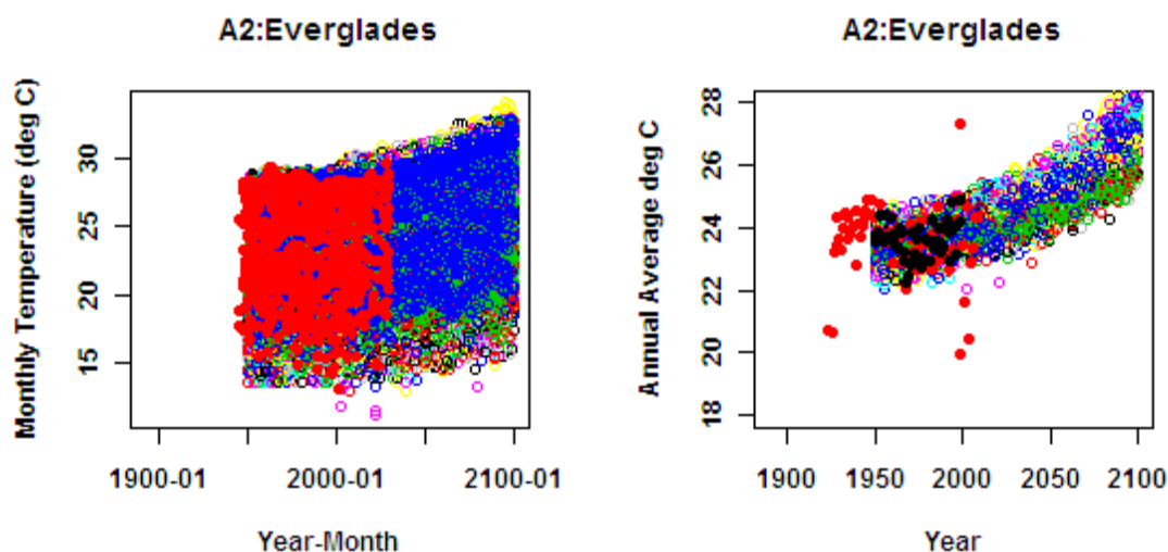
Figure 38. Monthly (left) and annual temperature patterns of BCSD models corresponding to the A2 scenario for the Everglades location. Also shown are historical observed data for the same location (red dots) and historical simulated data (black dots).
