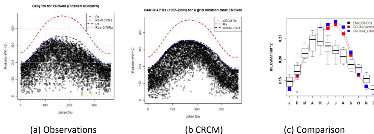
Figure 53. (a) Observed Seasonal patterns of incoming solar radiation at the ENR 308 stations, (b) CRCM model output for a cell nearest to that station, (c) observed vs. model data comparison.
