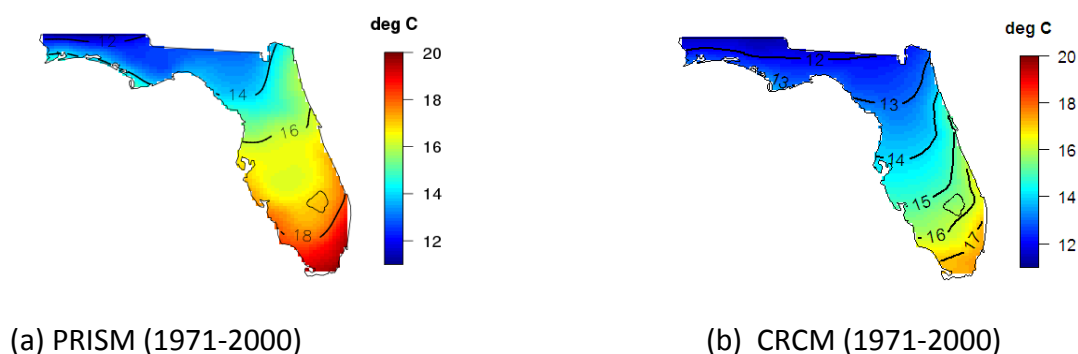
Figure 48. Comparison of (a) PRISM data, based on observations, and (b) the CRCM model output for average daily minimum temperature over the period 1971-2000.
