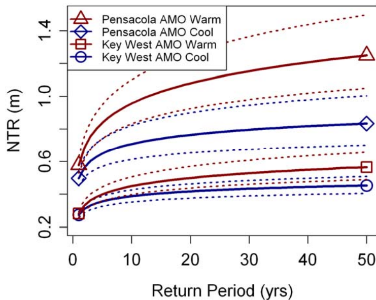
Figure 64. NTR (storm surge) return levels at Key West and Pensacola as a function of two AMO index regimes: Warm (index > 0.1) and Cool (index < -0.1). Dotted lines are 95% confidence levels.
